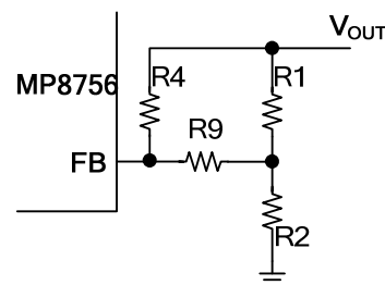
Figure 9: Equivalent DC Circuit
