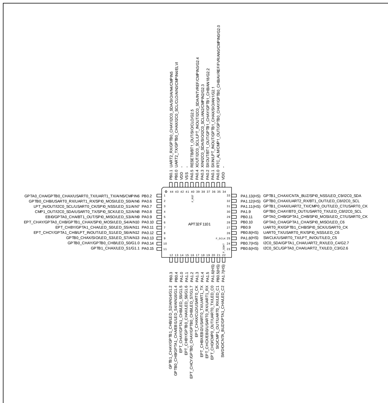
Figure 2-2 管脚定义图(44 LQFP)
