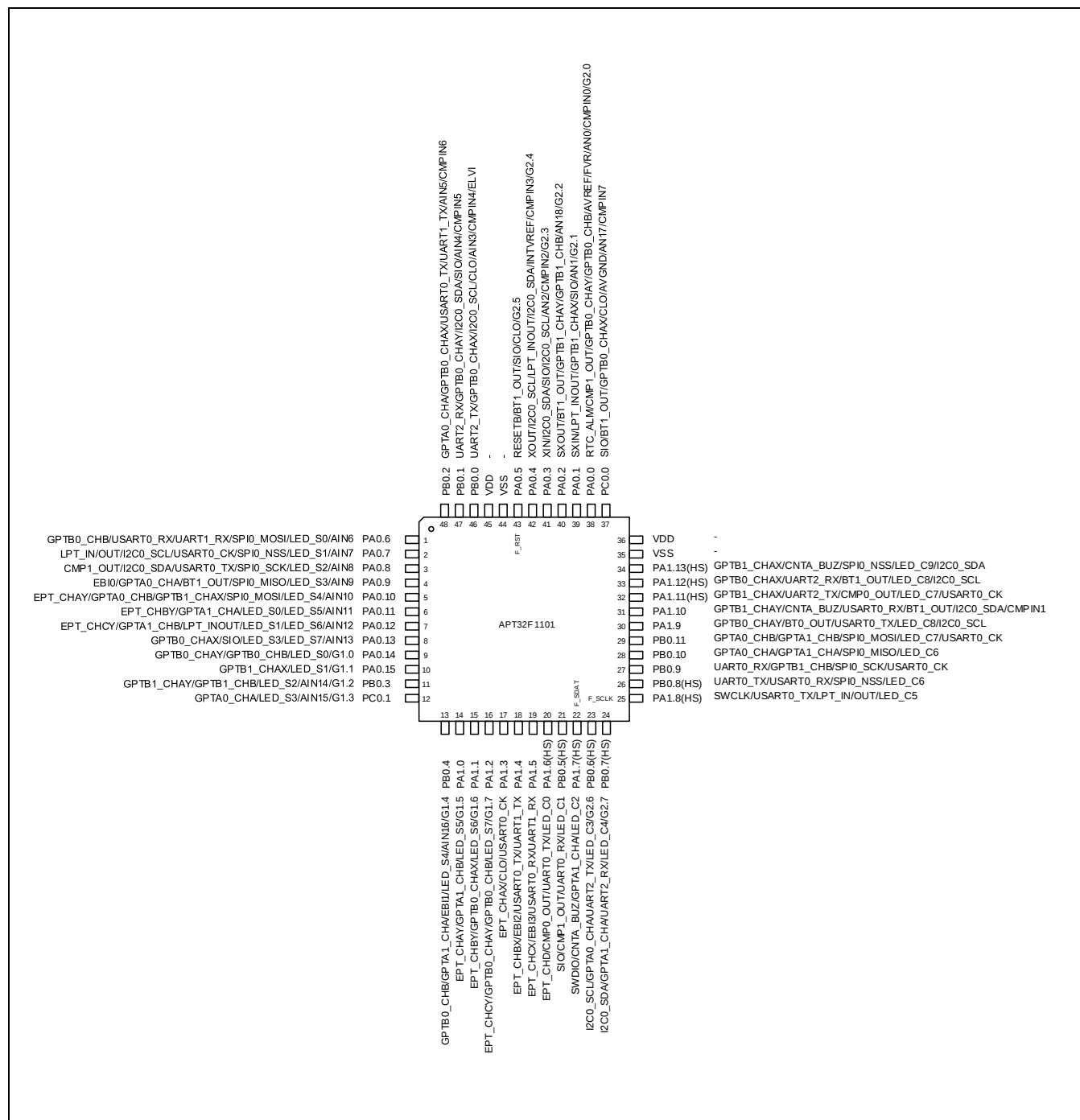
Figure 2-1 管脚定义图(48 LQFP/QFN)
