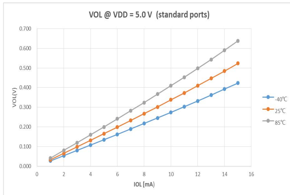
Figure 3-2 VOL(standard ports) 温度曲线
