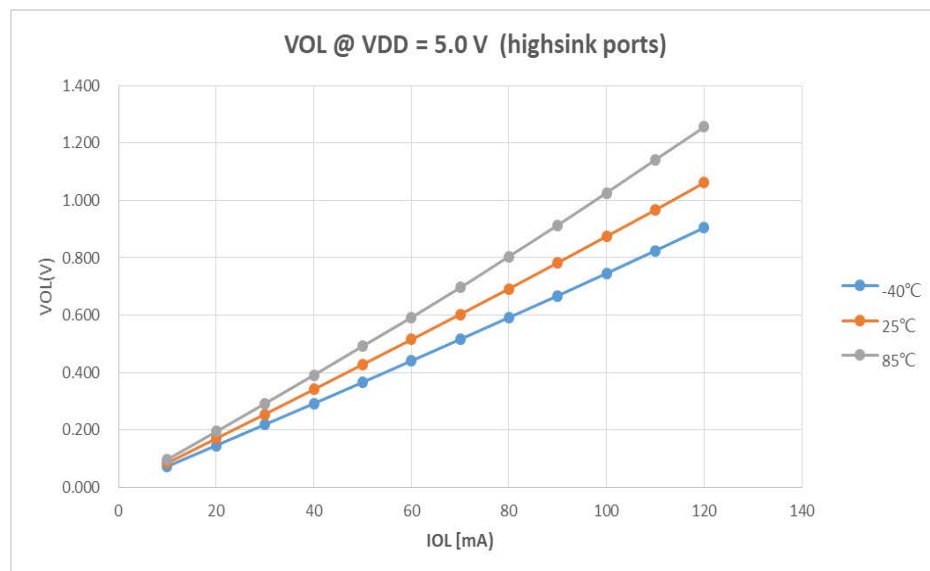
Figure 3-3 VOL(highsink ports) 温度曲线
